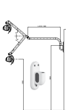
WANDADAPTION
