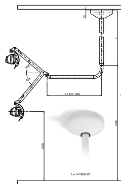
DECKENADAPTION
